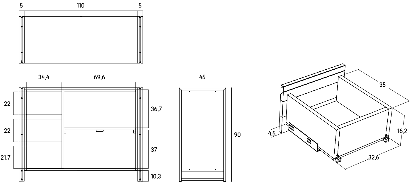
DRAWER DIMENSION
