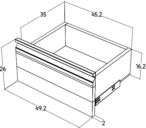
DRAWER DIMENSION
