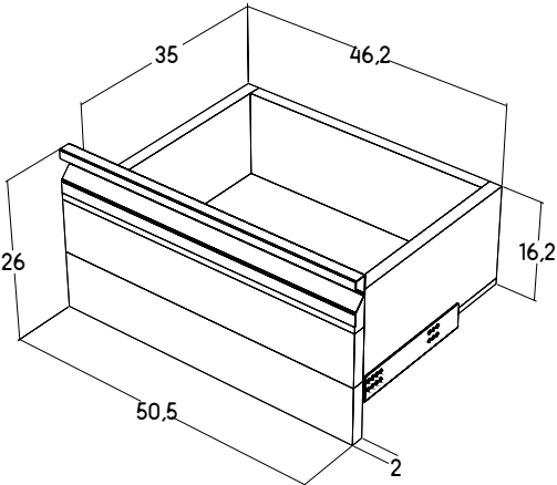
DRAWER DIMENSION
