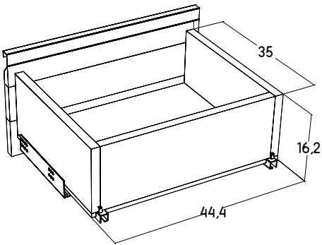
DRAWER DIMENSION
